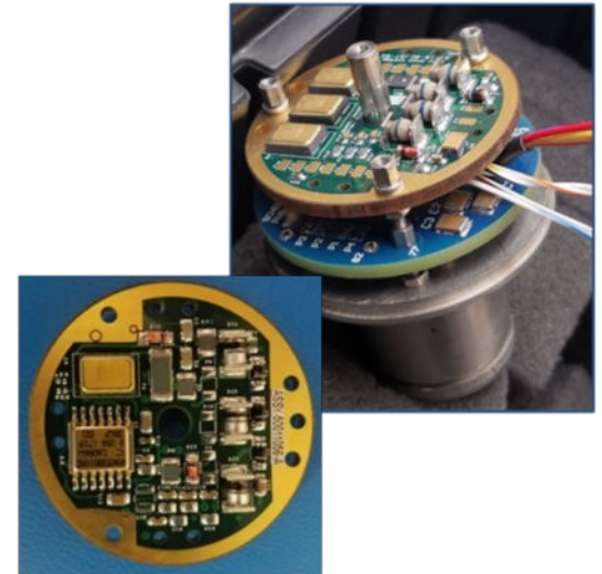
ECHO Controller and Commutator Board
